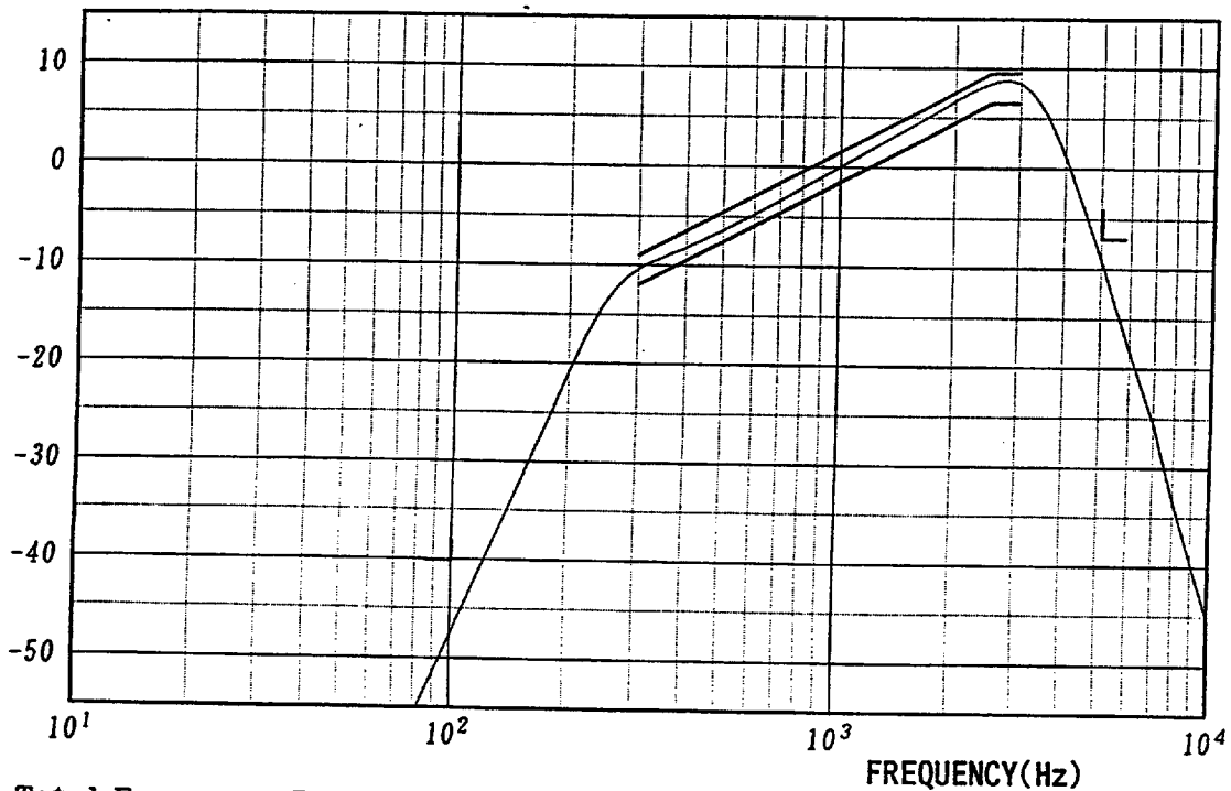
Fig.2 Total Frequency Response of Transmitter Section (FCONT="L")
