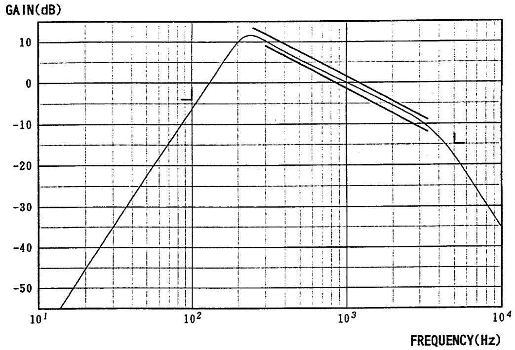
Fig.3 Total Frequency Response of Receiver Section
