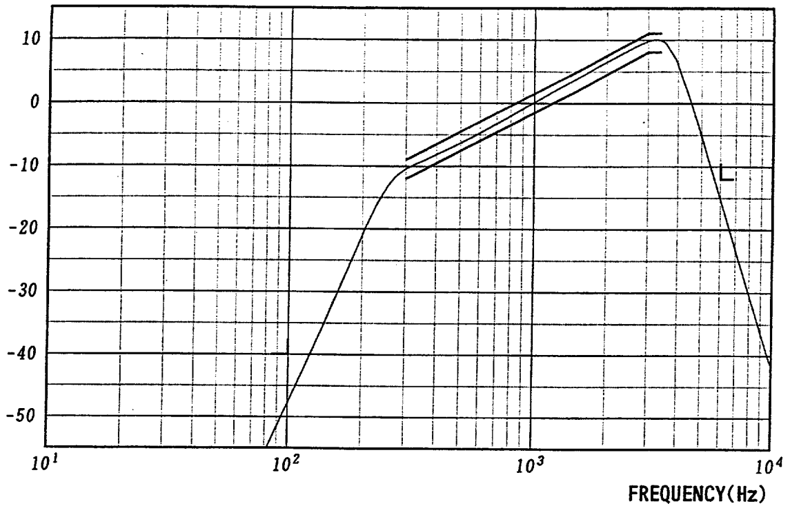
Fig.1 Total Frequency Response of Transmitter Section (FCONT="H")
