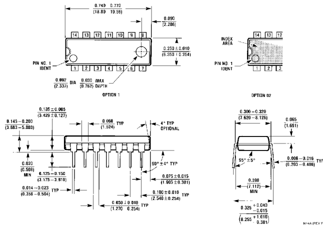
Dual-In-Line Package (N) Order Number CD4066BMN or CD4066BCN NS Package Number N14A
