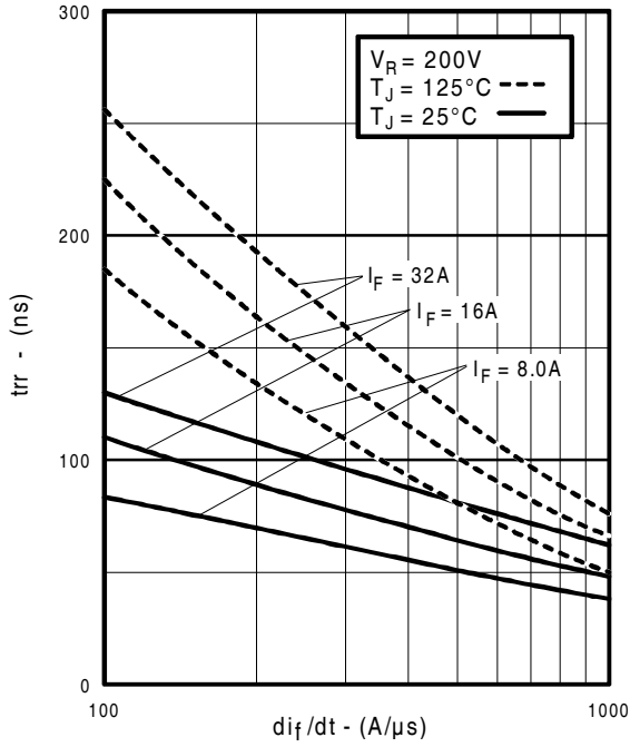
Fig. 14 - Typical Reverse Recovery vs. d i_f / d t
