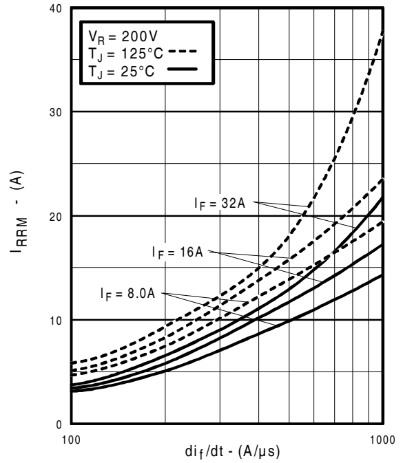
Fig. 15 - Typical Recovery Current vs. d i_f / d t
