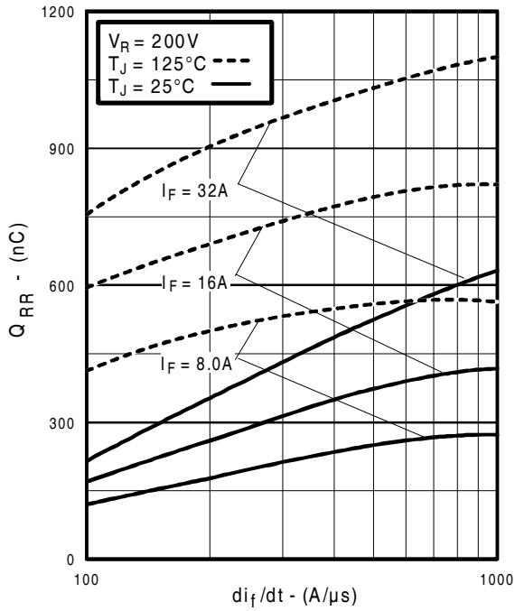
Fig. 16 - Typical Stored Charge vs. d i_f / d t
