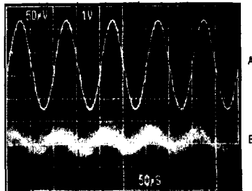
A = REF1, 1V/div (4Vp-p) B = OUT1, 50µV/div, UNLOADED FILTER PASSBAND = 1kHz to 100kHz, DAC CODE = 00 HEX
