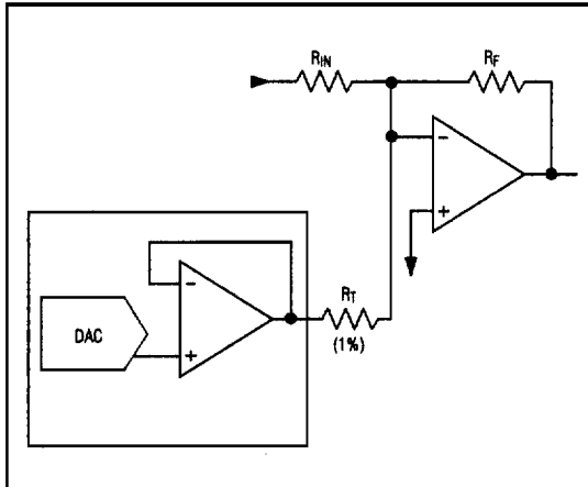
Figure 15a. Typical Trimming Circuit
