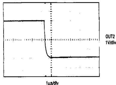
MAX520 NEGATIVE SETTLING TIME
