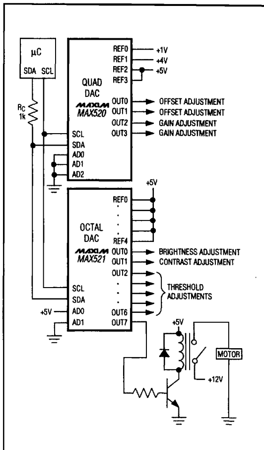
Figure 2. Typical Application Circuit
