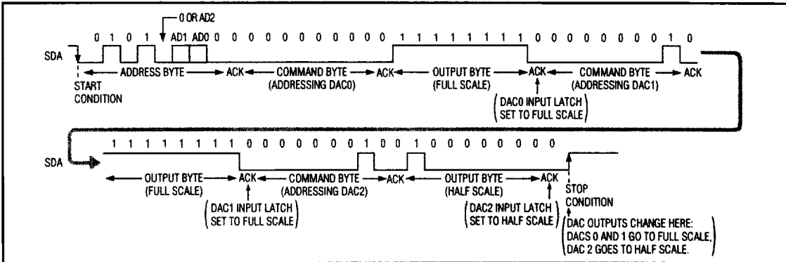
Figure 7. Setting DAC Outputs
