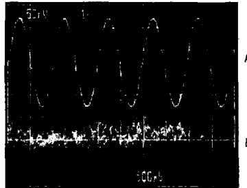
A = REF1, 1V/div (4Vp-p) B = OUT1, 50µV/div, UNLOADED FILTER PASSBAND = 100Hz to 10kHz, DAC CODE = 00 HEX
