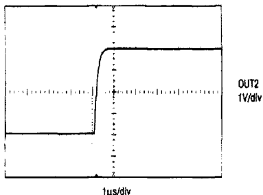
MAX520 POSITIVE SETTLING TIME
