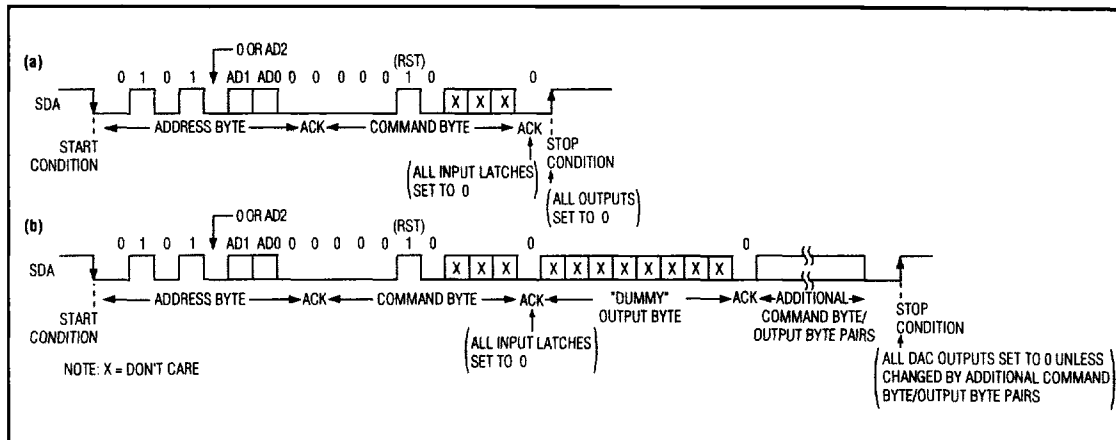
Figure 10. Resetting DAC Outputs
