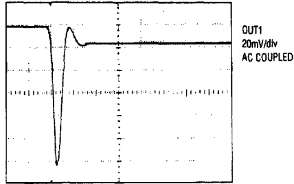
500ns/div REF1 = 5V, DAC CODE = 80 HEX to 7F HEX
