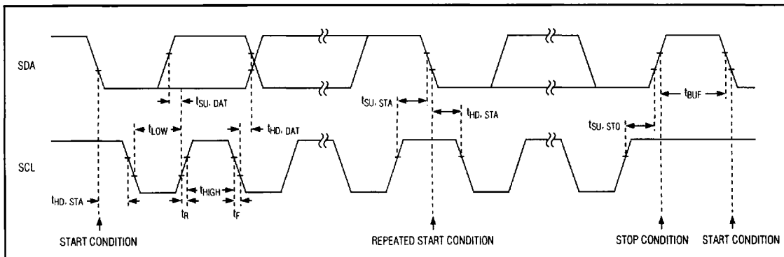
Figure 1. 2-Wire Serial-Interface Timing Diagram
