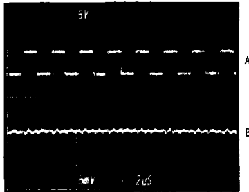
A = SCL, 400kHz, 5V/div B = OUT1, 5mV/div REF1 = 5V, DAC CODE = 7F HEX
