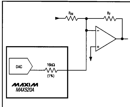
Figure 15b. MAX520A Trimming Circuit
