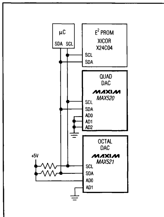
Figure 11. Typical I 2 C Application Circuit
