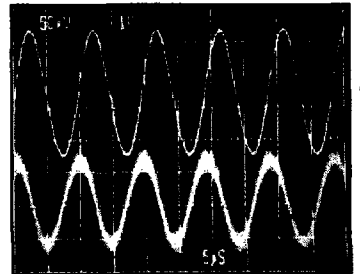
A = REF1, 1V/div (4Vp-p) B = OUT1, 50µV/div, UNLOADED FILTER PASSBAND = 10kHz to 1MHz, DAC CODE = 00 HEX
