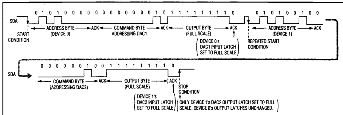
Figure 12. Repeated START Conditions
