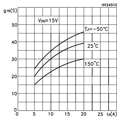
Figure 5: Transconductance
