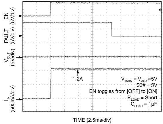
Main Turn-On into Short
