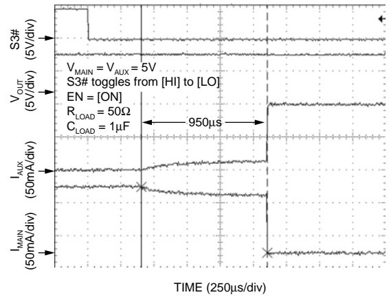
Main-to-AUX Cross Conduction
