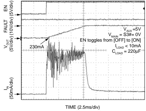
AUX Inrush Current into Large C_LOAD
