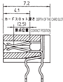
奇数ピン位置 POSITION OF ODD-NUMBERED PINS
