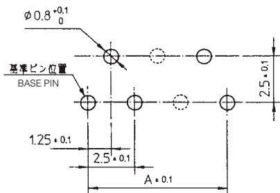
基板穴明寸法 (コネクタ搭載面) RECOMMENDED P.C. BOARD LAYOUT (View from connector mounting side) (適用基板厚 t=1~1.6) APPLICABLE BOARD THICKNESS
