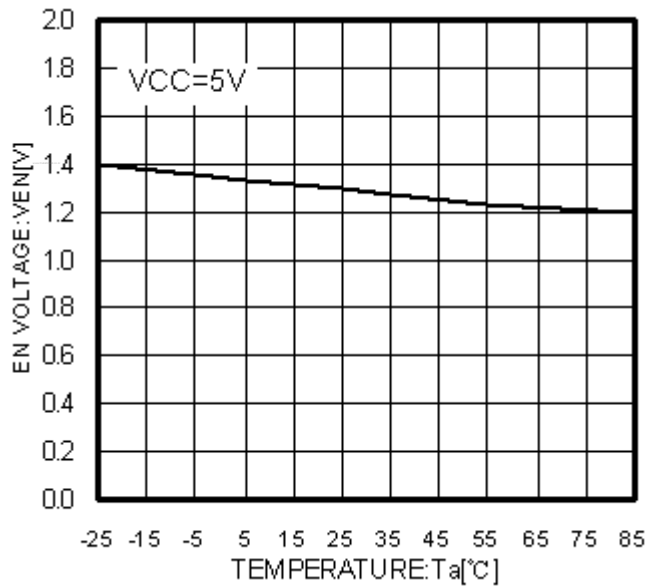
Fig.32 T_a - V_{EN}
