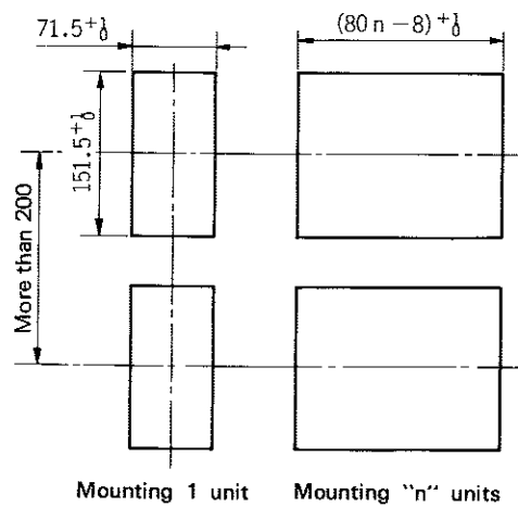
Vertical mounting
