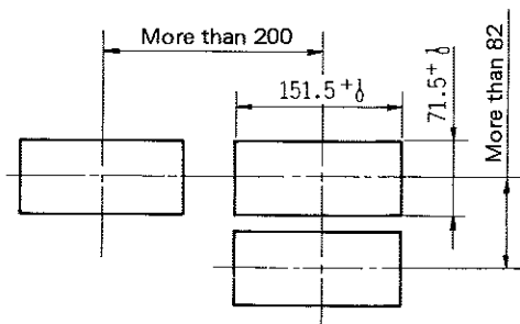
Horizontal mounting
