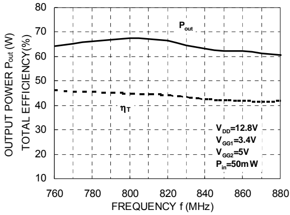
OUTPUT POWER, TOTAL EFFICIENCY, versus FREQUENCY
