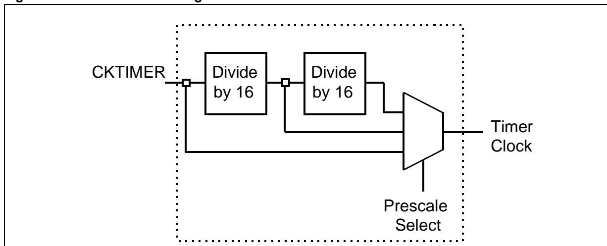
Figure 12. Pre-scaler block diagram
