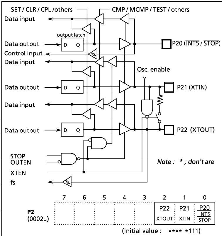
Figure 2-5. Port P2
