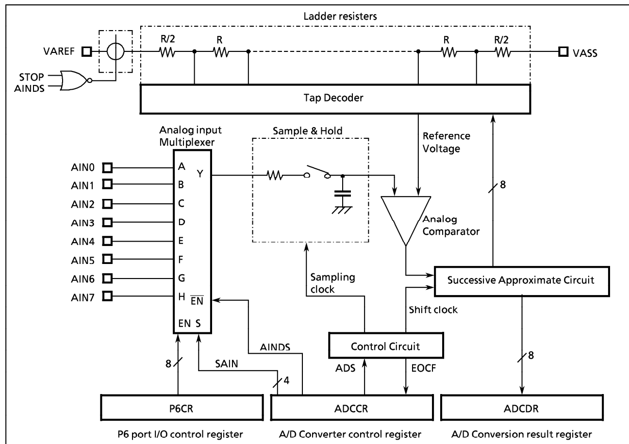
Figure 2-46. A/D Converter
