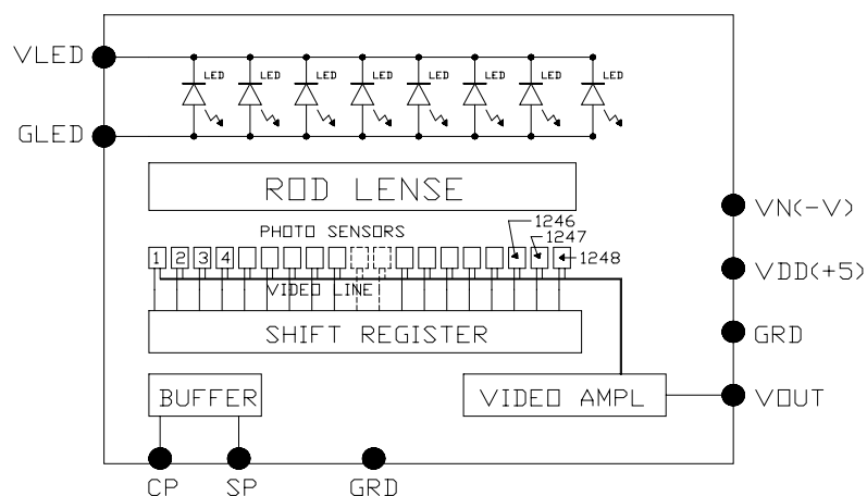
Figure 2: AMIS-710625-A6 Module Block Diagram
