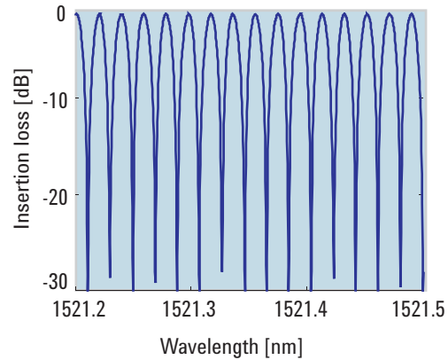
Figure 7. Loss curve of a DPSK demodulator.
