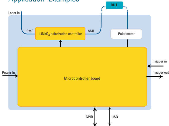
Figure 3. Instrument setup
