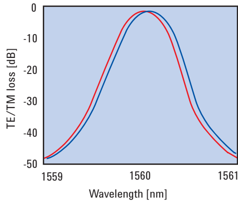
Figure 4. Polarization-dependent wavelength shift (PD-A) of a filter.
