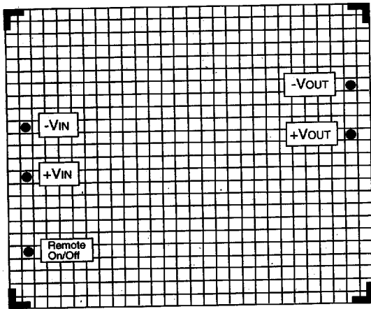
BOTTOM VIEW - SINGLE OUTPUT MODELS
