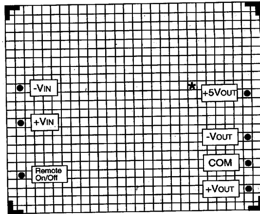
BOTTOM VIEW - DUAL AND TRIPLE OUTPUT MODELS
