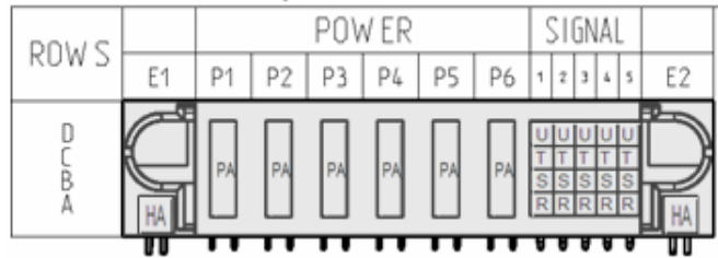
Connector: FCI (51732-020 LF)
