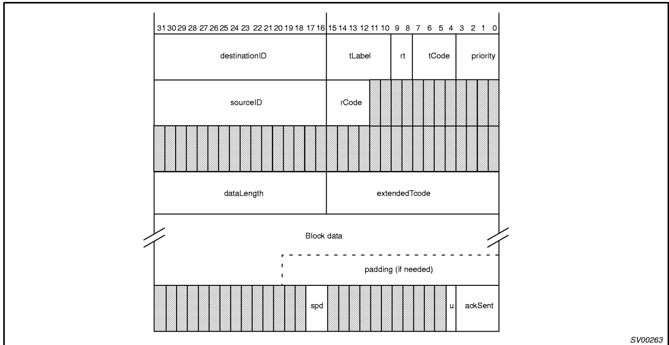
Figure 18. Block Read or Lock Response Receive Format
