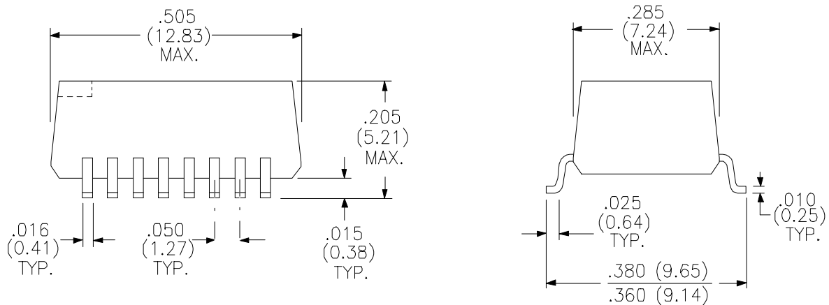
Physical Dimensions inches (mm)
