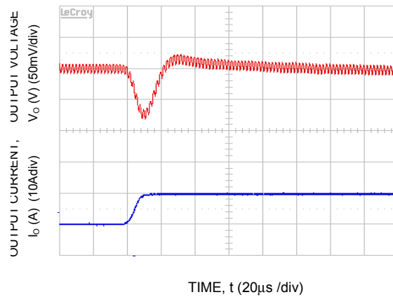
Figure 34. Transient Response to Dynamic Load Change from 50% to 100% at 12Vin, C_{Out}=8x47\mu F , C_{Tune}=1500pF & R_{Tune}=220\text{ ohms}
