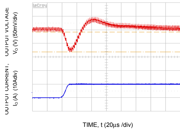
Figure 28 Transient Response to Dynamic Load Change from 50% to 100% at 12V in , C out = 5x47μF +1x330μF, C Tune =2200pF & R Tune =220 ohms
