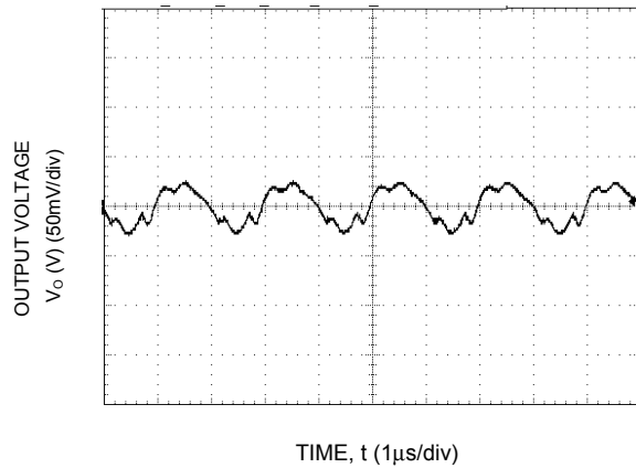
Figure 27. Typical output ripple and noise (C O =2x47μF ceramic, V IN = 12V, I o = I o,max ).
