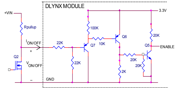
Figure 39. Circuit configuration for using positive On/Off logic.
