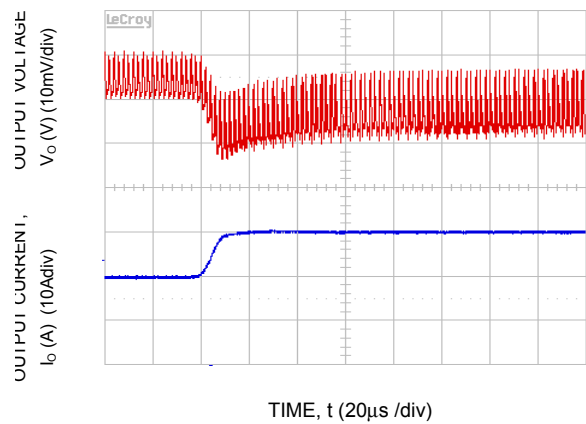
Figure 4. Transient Response to Dynamic Load Change from 50% to 100% at 12Vin, C_{out} = 1 \times 47\mu\text{F} + 11 \times 330\mu\text{F} C_{Tune}=47\text{nF} , R_{Tune}=178\text{ ohms}
