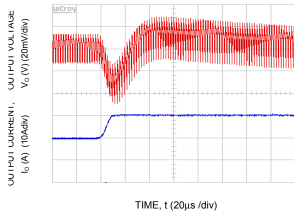
Figure 16. Transient Response to Dynamic Load Change from 50% to 100% at 12Vin, C_{out}= 2x47\mu F +3x330\mu F , C_{Tune}=5600pF & R_{Tune}=220 ohms
