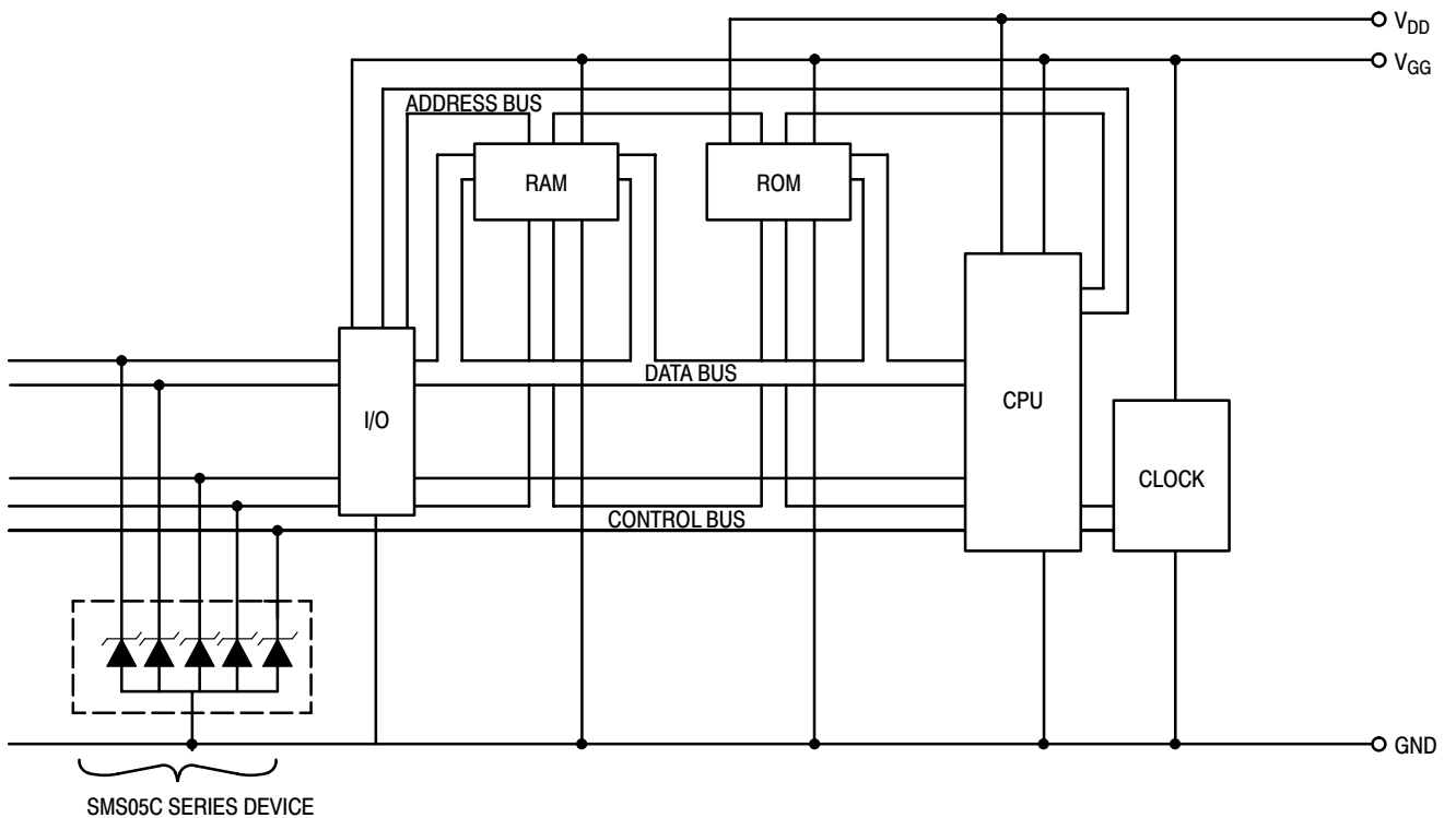
Figure 8. Microprocessor Protection
