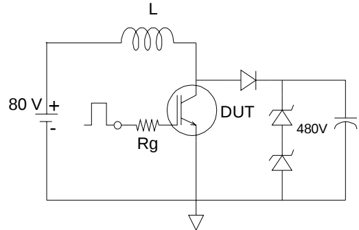
Fig.C.T.2 - RBSOA Circuit
