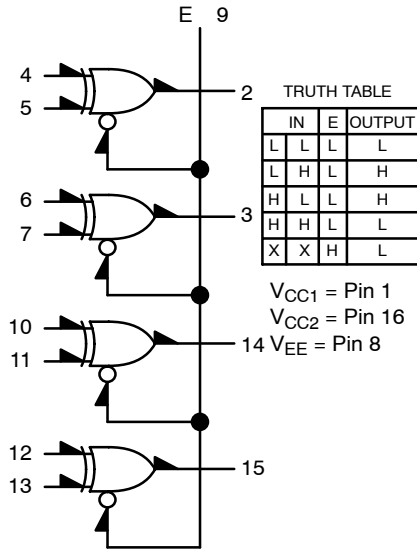
Figure 1. Logic Diagram
