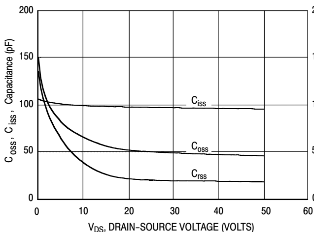
Figure 6. Capacitance versus Voltage
