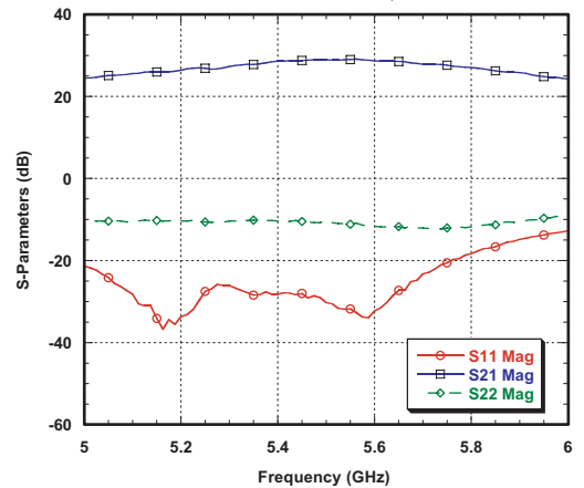
RMPA2550 S-Parameters 5.0 GHz Band T=25C VM, VC=3.3V
