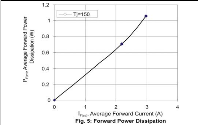
Fig. 5: Forward Power Dissipation
