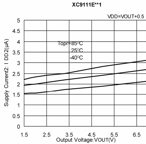
(7) No Load Input Current vs. Output Voltage
