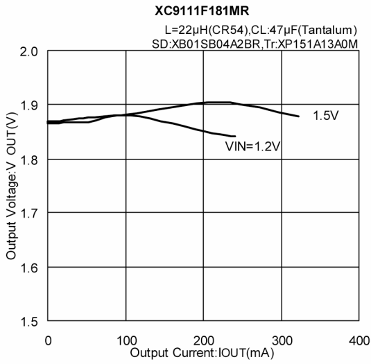
(1) Output Voltage vs. Output Current (Continued)
