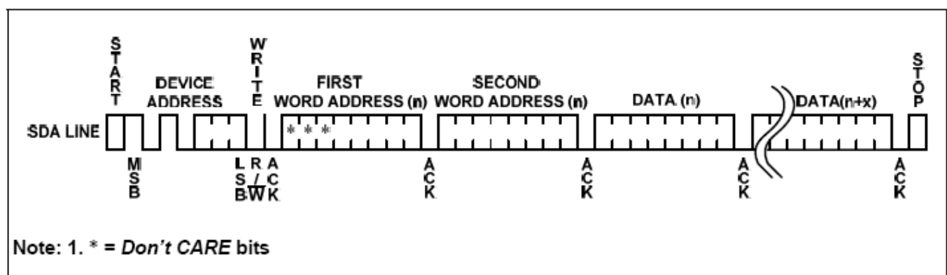
Figure 9 · Page Write
