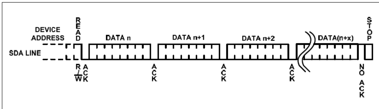
Figure 12 · Sequential Read
