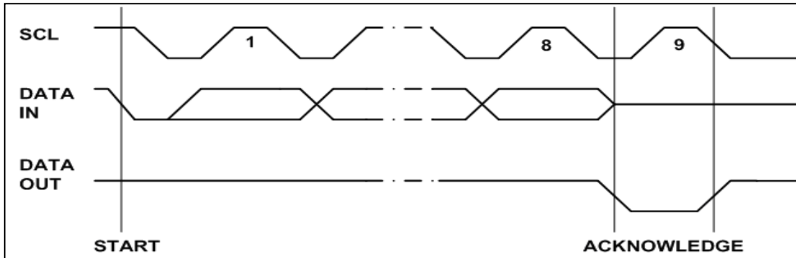
Figure 6 · Output Acknowledge
