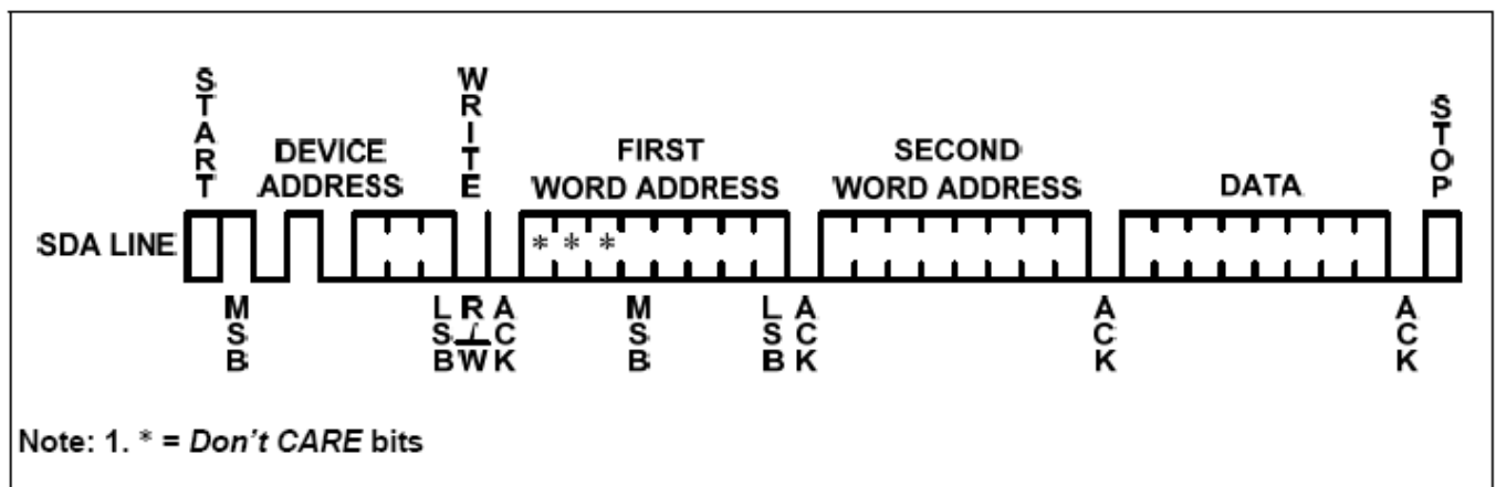
Figure 8 · Byte Write
