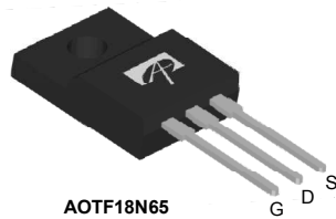
TO-220F
