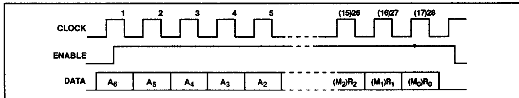
Fig. 4 Timing diagram showing programming details
