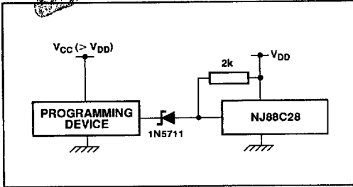
Fig. 7 Suggested programming circuit
