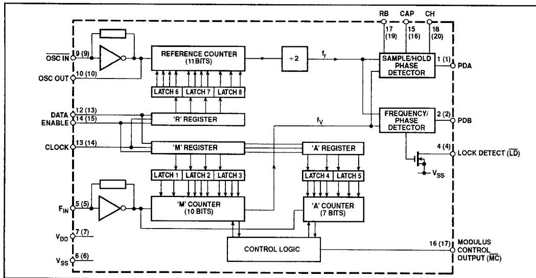
Fig.2 block diagram (NP pinout shown in brackets)
