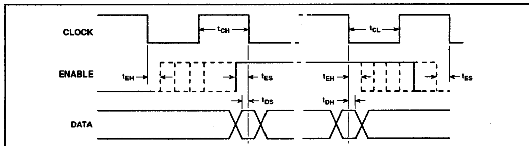
Fig. 3 Timing diagram showing timing periods required for correct operation
