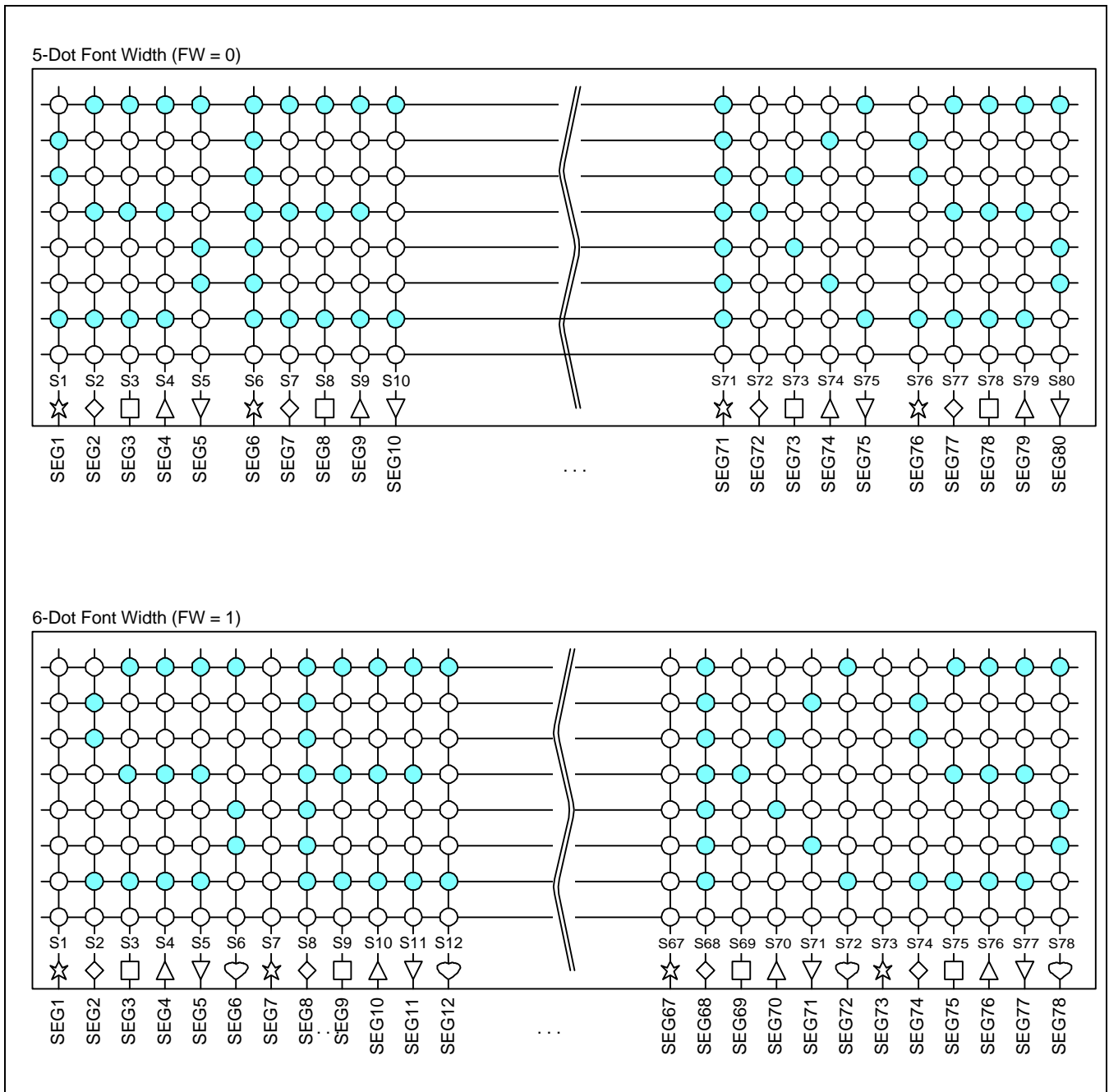
Figure 8. Relationship between SEGGRAM and Segment Display
