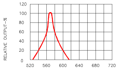
Fig.2 SPECTRAL RESPONSE
