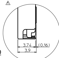
DETAIL B (5:1)
