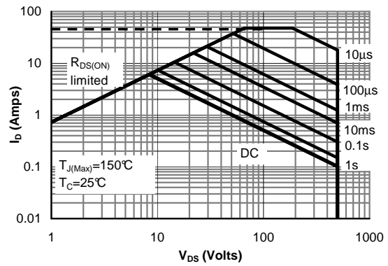
Figure 10: Maximum Forward Biased Safe Operating Area for AOTF13N50 (Note F)
