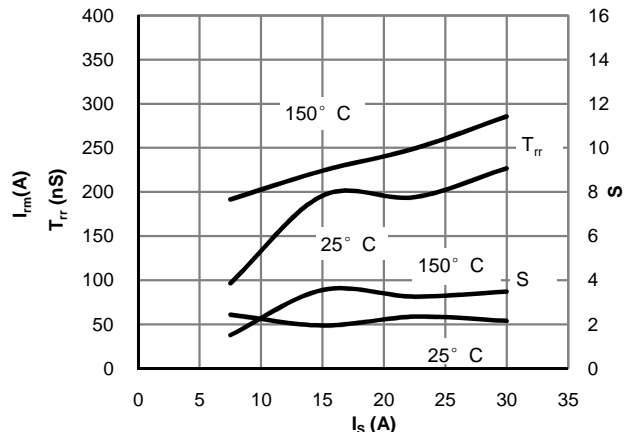
Fig 23: Diode Reverse Recovery Time and Softness Factor vs. Conduction Current ( V_{GE}=15V, V_{CE}=400V, di/dt=200A/\mu s )
