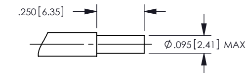
RECOMMENDED CABLE TRIM DIMENSIONS SCALE: 2:1
