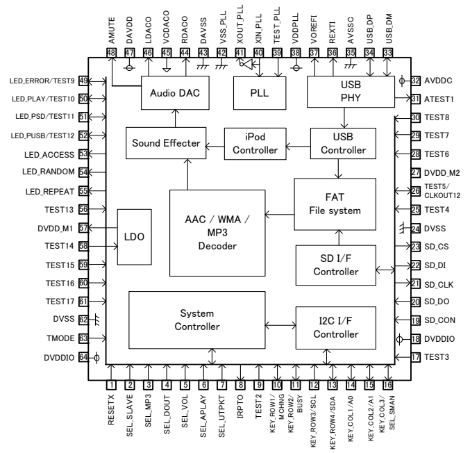
Figure 2. Block diagram
