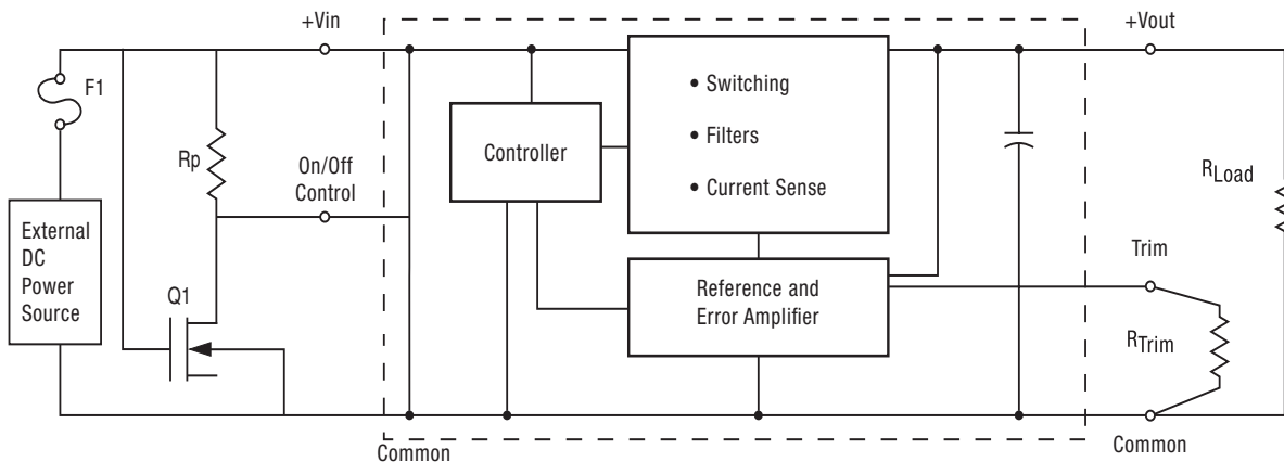
Figure 1. Connection Diagram
