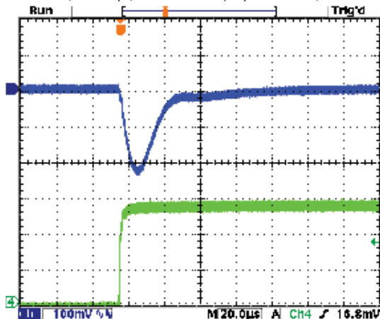
Step Load Transient Response (Vin=5.5V, Vout=3.3V, Cload=5x10µF X5R 0805 ceramic, total 50µF, Iout=0A to 1.5A) Top trace=Vout, Bottom trace=Iout
