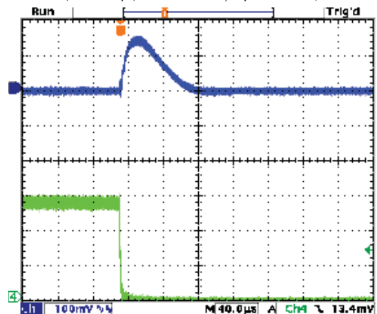
Step Load Transient Response (Vin=12V, Vout=1.8V, Cload=12x10µF X5R 0805 ceramic, total 120µF, Iout=1.5A to 0A) Top trace=Vout, Bottom trace=Iout
