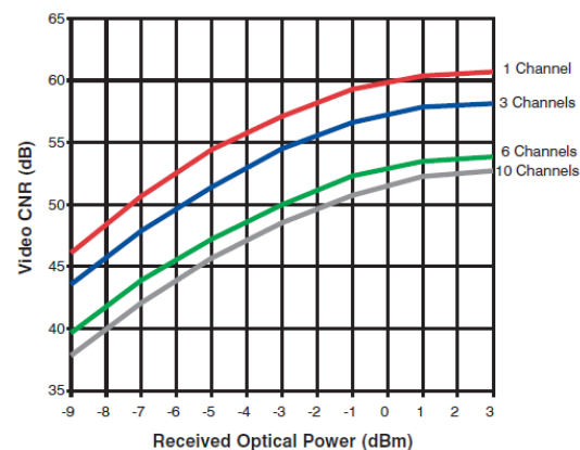
Carrier-to-Noise Performance:
