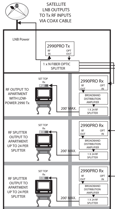
Typical MDU Application
