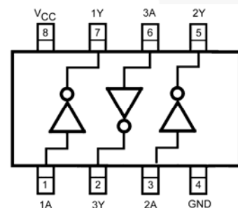
Figure 2. Connection Diagram
