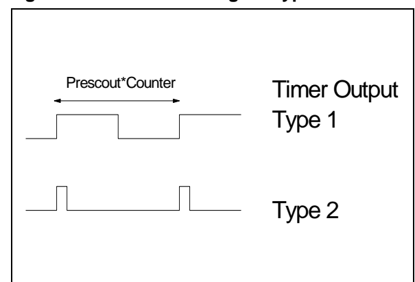
Figure 10.3 TIMEROUT Signal Type
