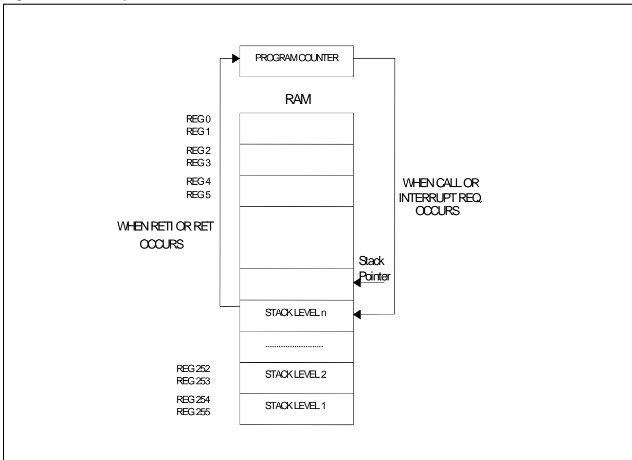
Figure 2.4 Stack Operation
