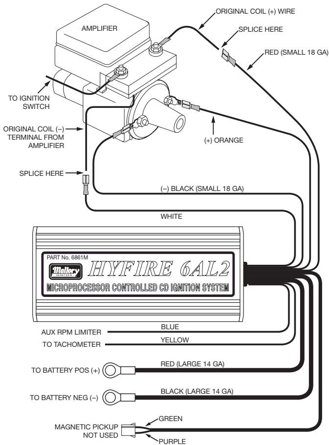
FIGURE 23 Installing the HYFIRE® 6AL2 with a Typical Import Application
