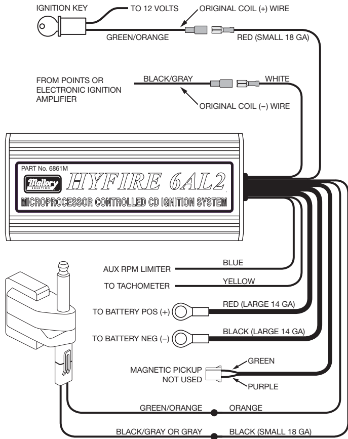
FIGURE 22 Installing the HYFIRE® 6AL2 with a Late Model Dodge (with 2-Pin Connector)
