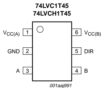
Fig 3. Pin configuration SOT363 (SC-88)
