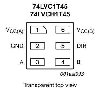
Fig 5. Pin configuration SOT891
