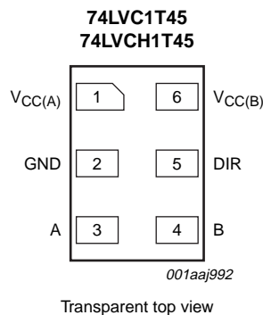
Fig 4. Pin configuration SOT886 (XSON6)
