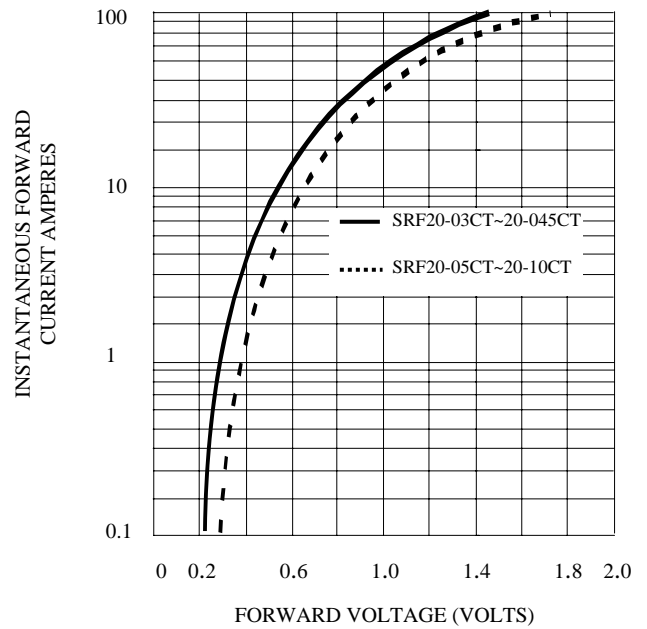
FIG. 4 - TYPICAL FORWARD CHARACTERISTIC PER LEG
