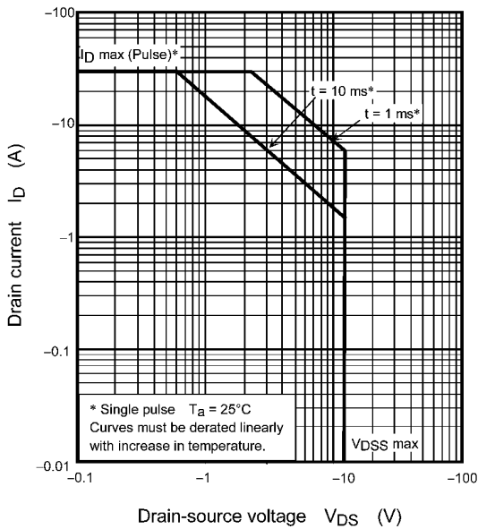
Fig. 7.15 Safe Operating Area
