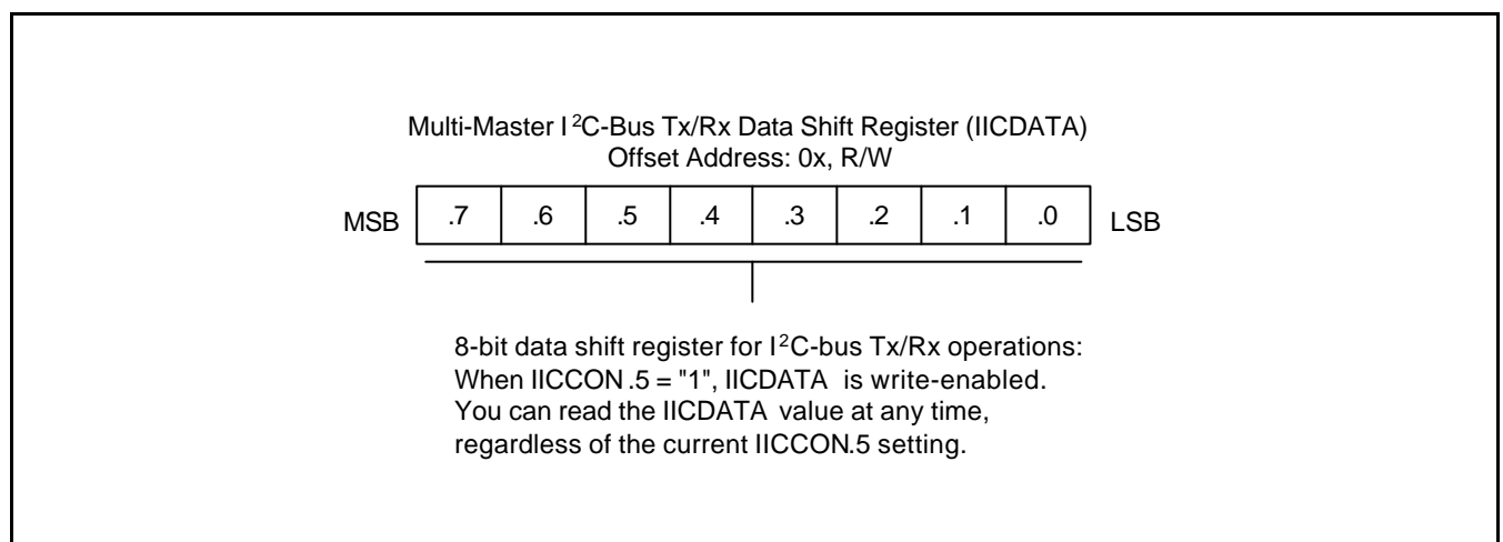
Figure 21-2. Multi-Master I 2 C-Bus Tx/Rx Data Register (IICDATA)
