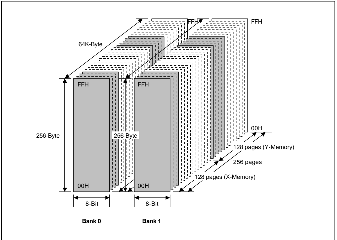
Figure 2-2. Data Memory Map
