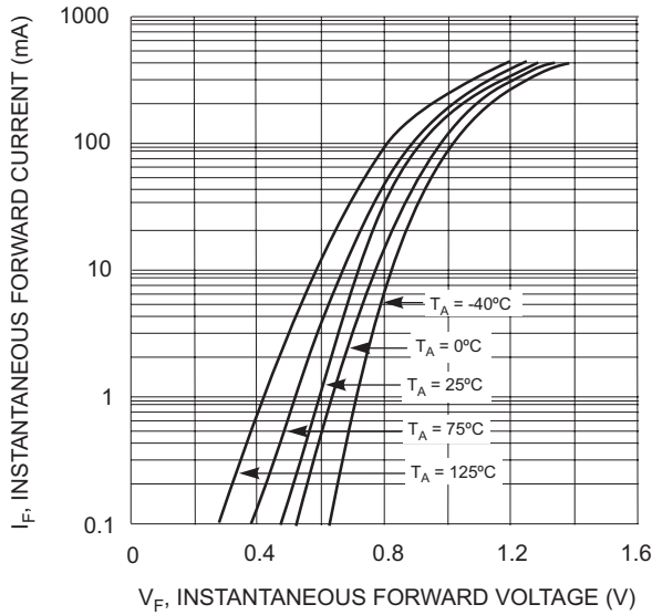
Fig. 7 Typical Forward Characteristics
