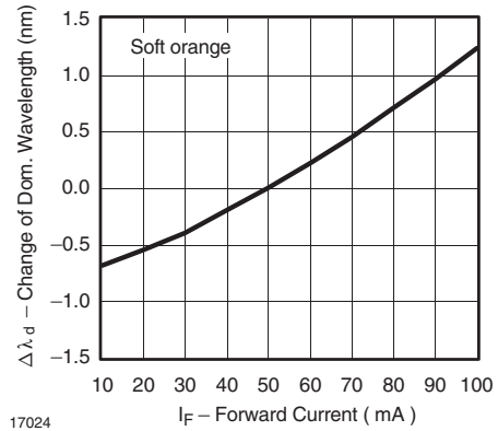
Figure 22. Change of Dominant Wavelength vs. Forward Current
