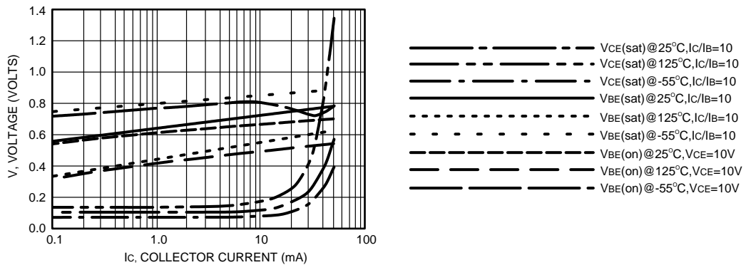
Figure 4. "ON" Voltages
