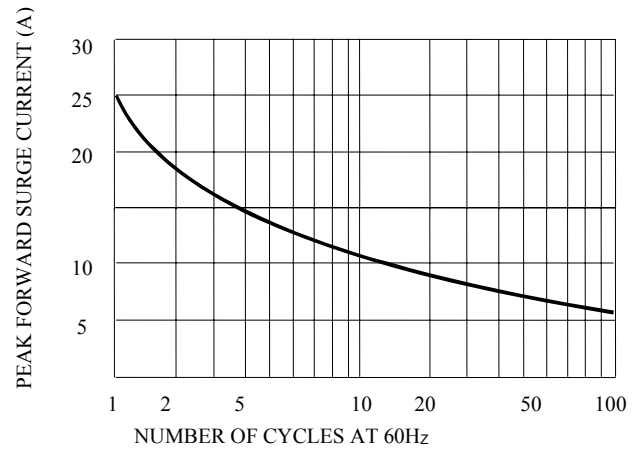
FIG. 4 - MAXIMUM NON-REPETITIVE
